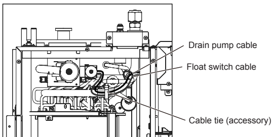
(③ Bottom view: Drain pump side)
