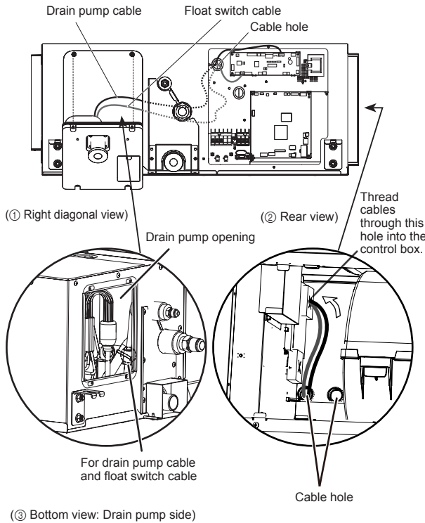
(③ Bottom view: Drain pump side)
