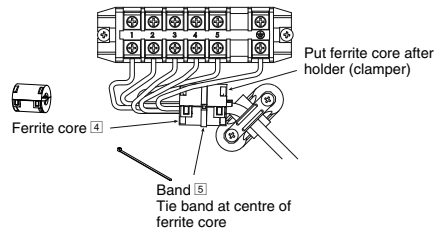
TERMINAL BOARD VIEW
