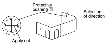
DETAIL OF CONNECTING CABLE GUIDING
