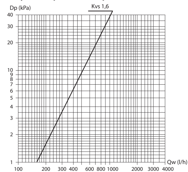
3 way valves pressure drop
