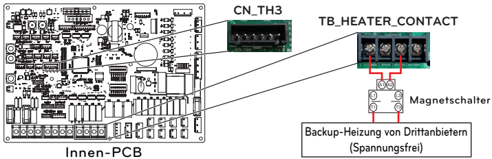
Innen-PCB
