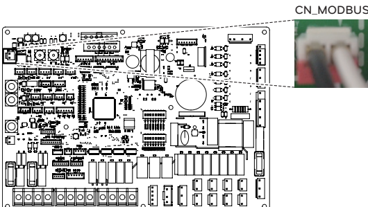
Innen-PCB
