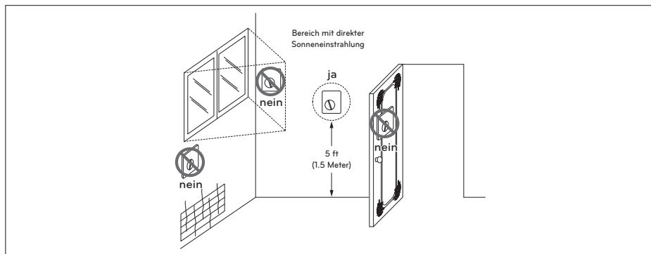
Thermostat
