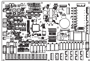
Innen-PCB
