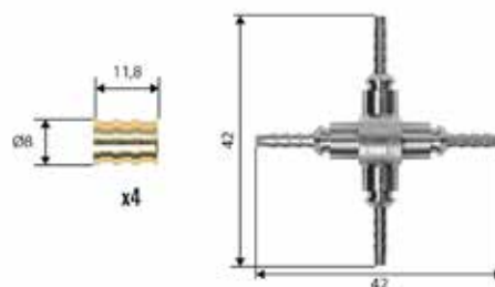
Cross Fitting
