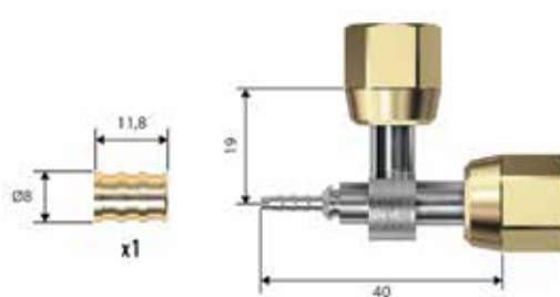
"T" Fitting With 2 Females 1/4 SAE At 90°
