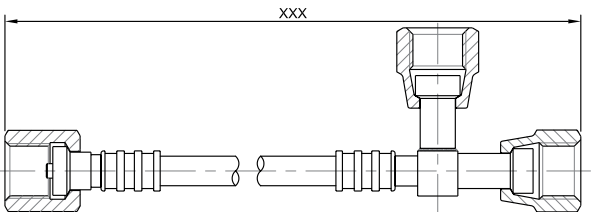
Straight Female 1/4 With Valve Opener + T With 2 Females 1/4 at 90°
