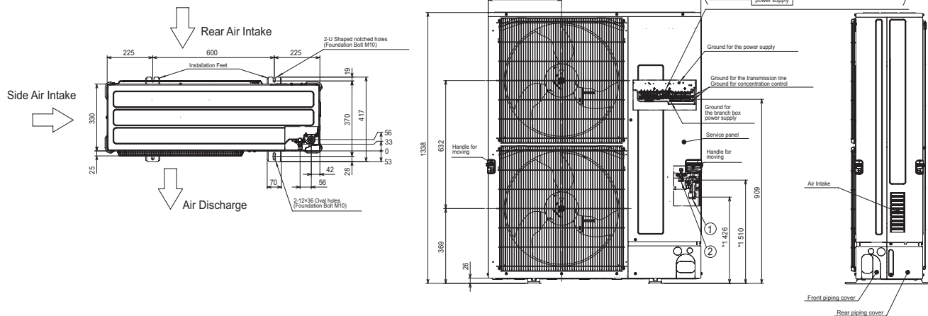
PUMY-P112-140VKM/YKM
