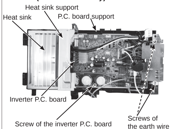
Photo 5 (Inverter assembly)
