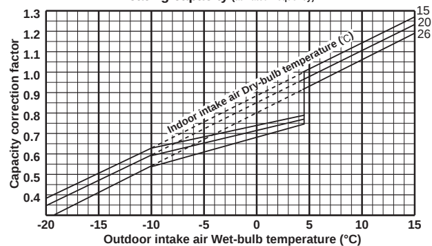
Heating capacity (at Rated frequency)
