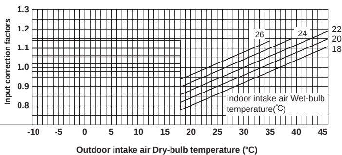
Total input (Cooling : at Rated frequency)
