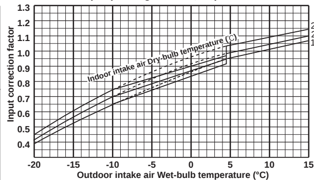
Total input (Heating : at Rated frequency)
