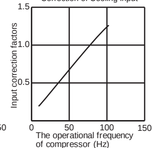
Correction of Cooling input
