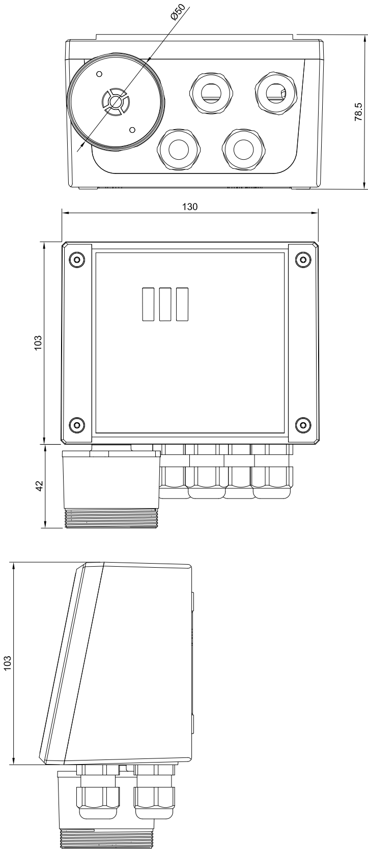
Built-in version
