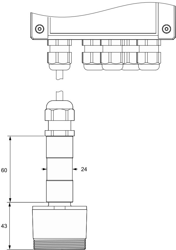
Remote version
