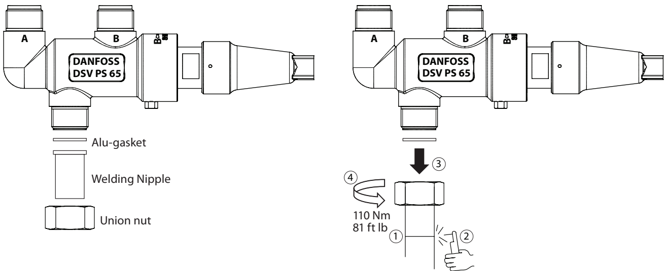
Fig. 1. DSV 10 inlet connection
