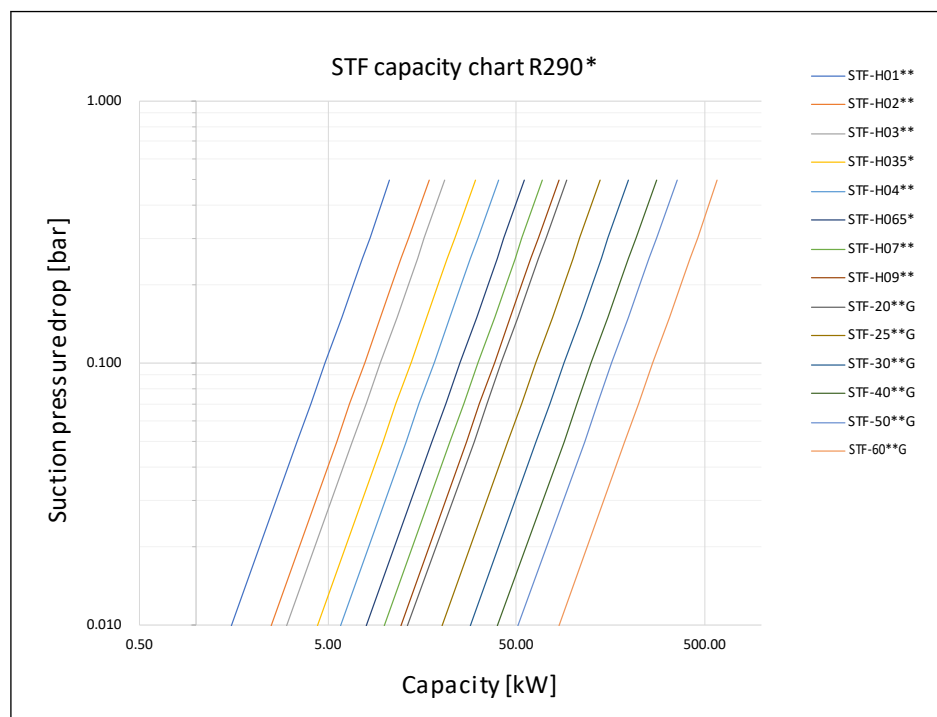
Figure 11: STF capacity chart R290
