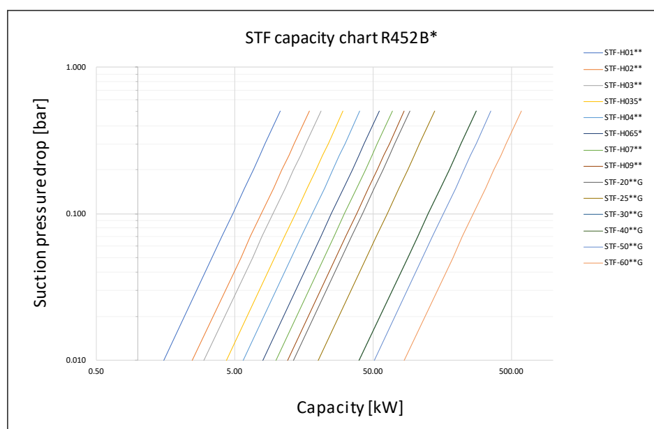
Figure 12: STF capacity chart R452B
