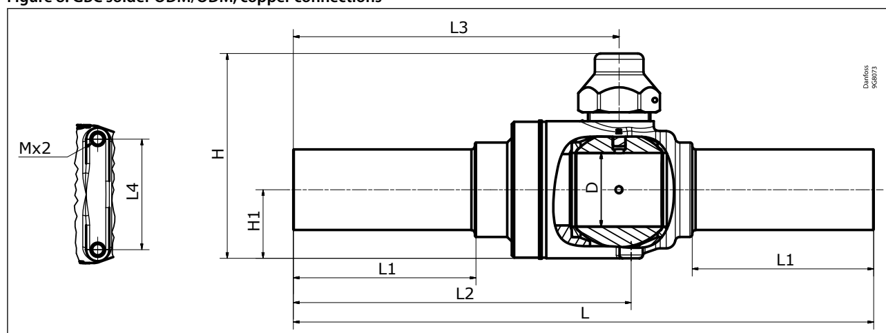
Figure 8: GBC solder ODM/ODM, copper connections
