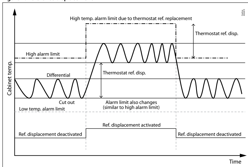
Figure 7: Reference displacement
