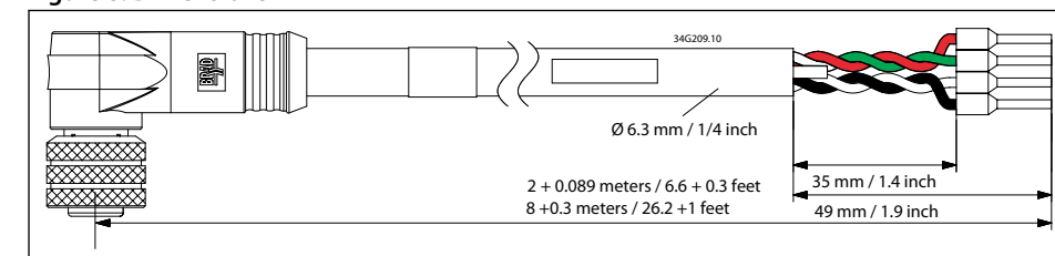
Figure 8: Dimensions
