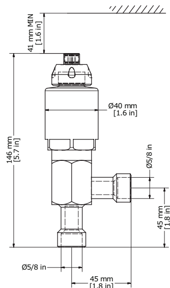
Danfoss DIM027H7250-00
