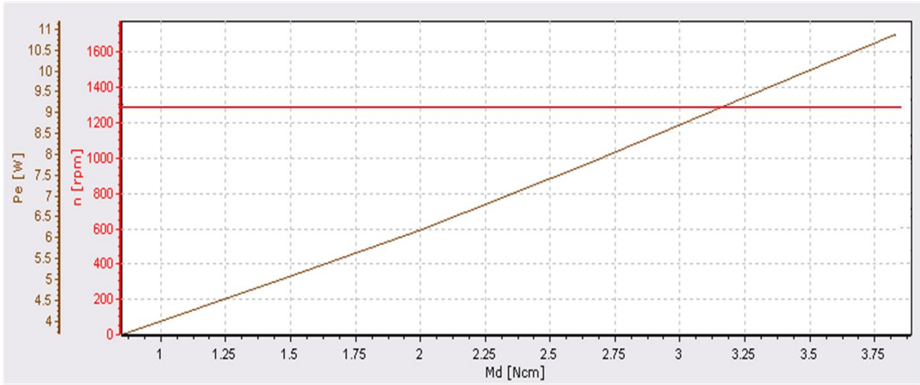
Curves:Speed(1300 rpm)
